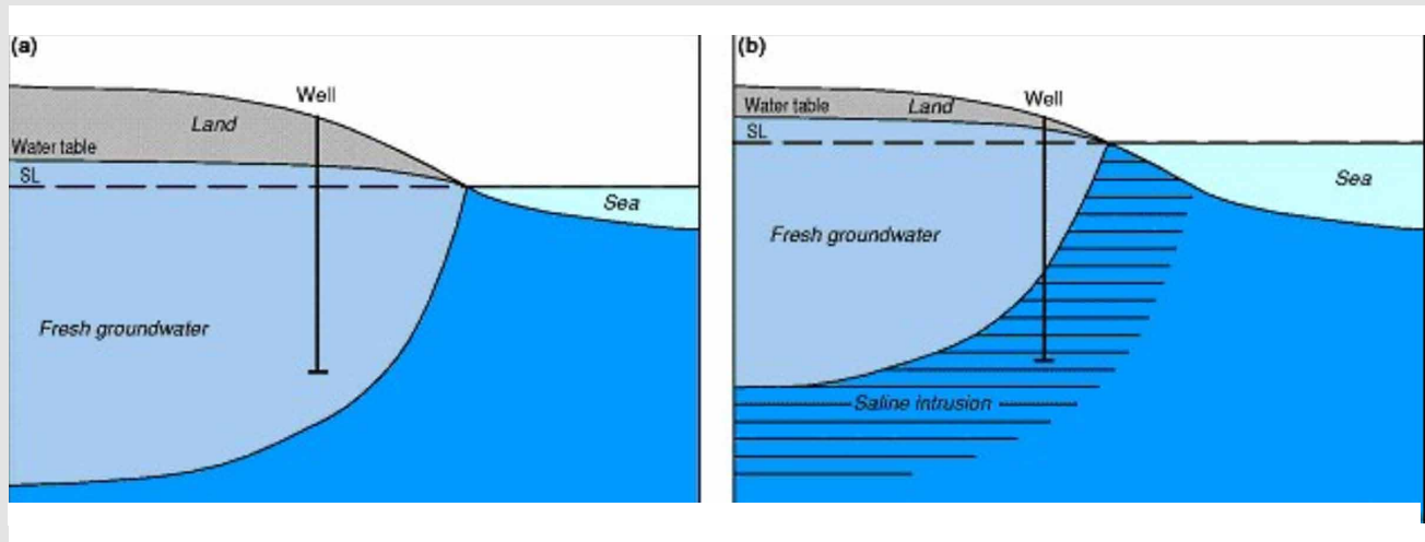
Figure 12.3: The impact of sea level rise on the saltwater-freshwater interface. (a) Water intake before sea level rise (b) water intake after sea level rise (Source: http://www.ozcoasts.gov.au/indicators/images/saltwater_freshwater.jpg ).
