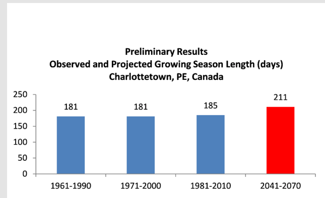
Figure 3.7: Historical observations and preliminary projections for the length of growing seasons in Charlottetown, PE, Canada (Source: Fenech, 2016).
