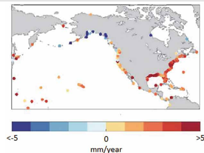
Figure 2.6: Differences in sea level trends globally based on full records (at least 30 years of data) measured and published for NOAA tide gauges through 2015 (Source: Sweet et al. , 2017).
