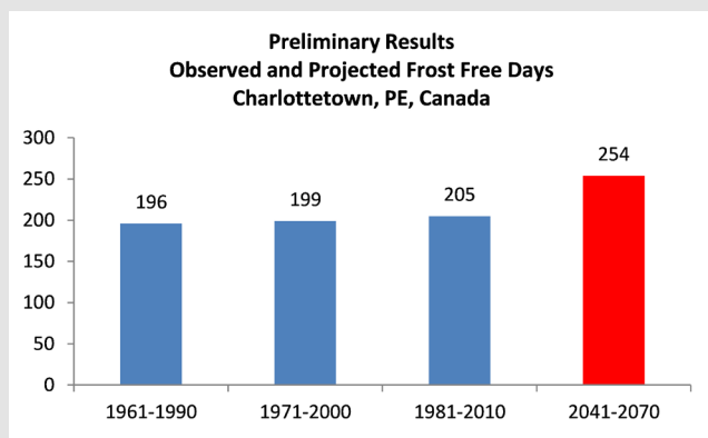
Figure 3.6: Historical observations and preliminary projections for the number of frost free days in Charlottetown, PE, Canada (Source: Fenech, 2016).
