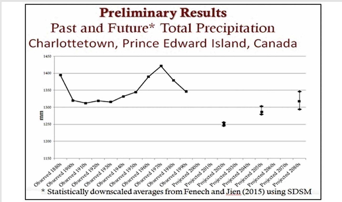
Figure 2.3: Historical observations and preliminary projection for total precipitation in Charlottetown, PE, Canada (Source: Fenech, 2016).
