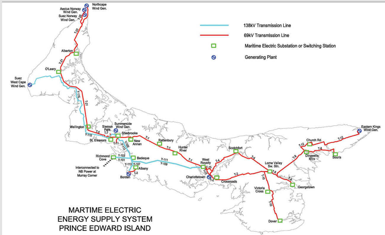
Figure 5.3: Maritime Electricity energy supply system map (Source: PEI Energy Commission, 2012)
