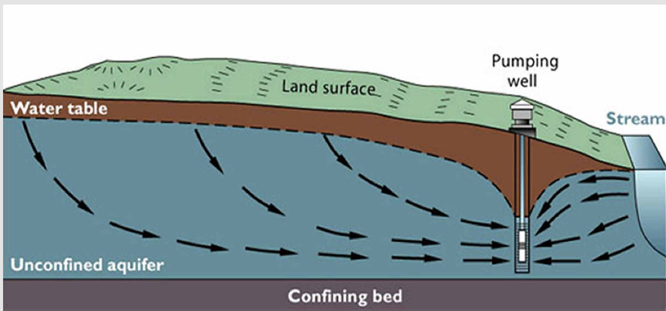
Figure 12.1: Groundwater and aquifer (Source: http://www.livinghistoryfarm.org/farminginthe50s/media/water1201.jpg ).
