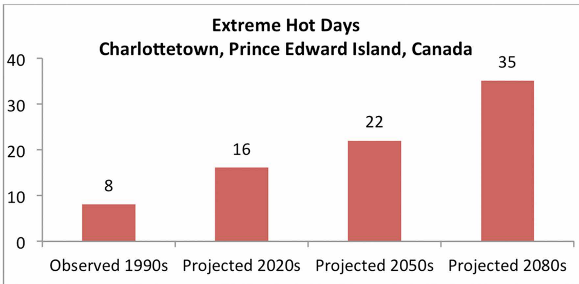
Figure 2.1: Projected number of days exceeding extreme hot temperatures (>27.5°C) for Charlottetown, PE, Canada (Source: Preliminary results from statistically downscaled averages from Fenech and Jien (2015) using SDSM).
