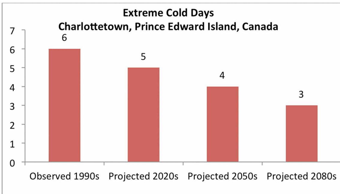
Figure 2.2: Projected number of days exceeding extreme cold temperatures (<-20°C) for Charlottetown, PE, Canada (Source: Preliminary results from statistically downscaled averages from Fenech and Jien (2015) using SDSM).
