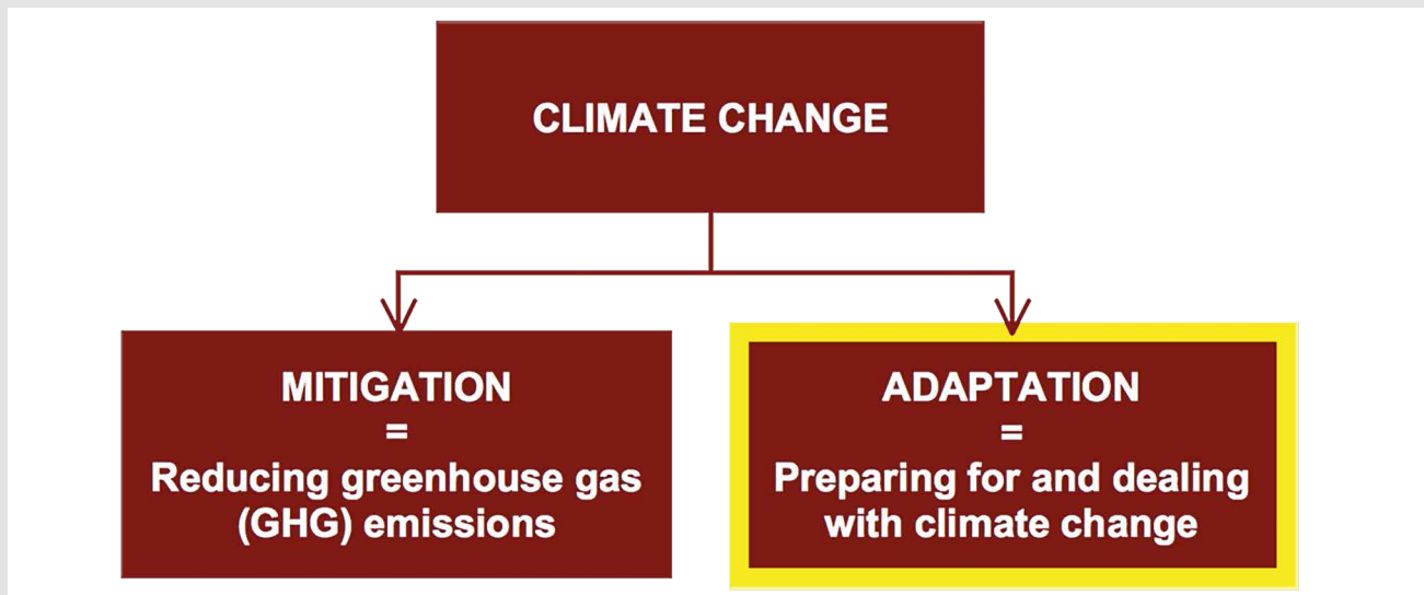
Figure 1.1: Climate change mitigation versus climate change adaptation.
