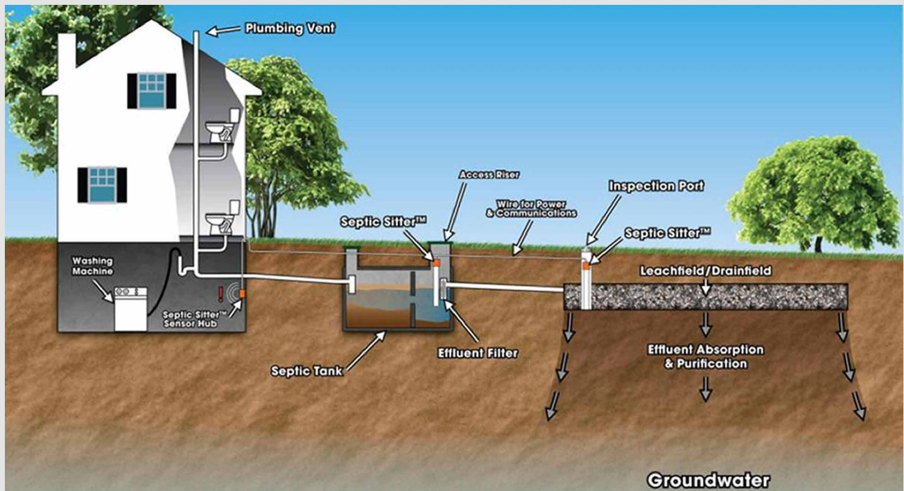
Figure 12.2: Septic system (Source: https://www.hi-techplumbingandair.com/wp-content/uploads/2015/10/Septic-Drainfield.jpg ).
