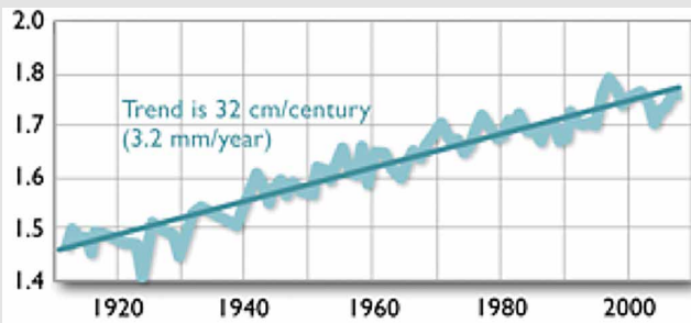
Figure 2.5: Observed increase in water level (metres above reference level on land) 1911–2008 at Charlottetown Harbour, PE, Canada (Source: Biodiversity Canada, 2014).
