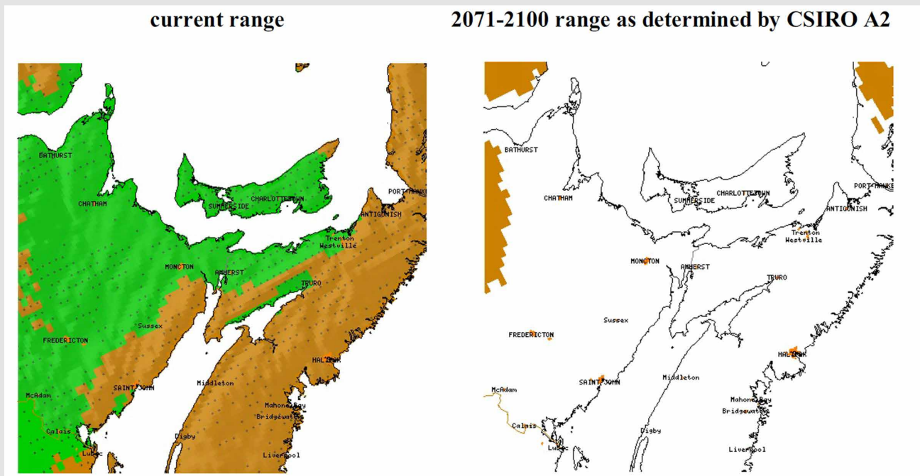
Figure 7.4: The current and potential range of white spruce using the CSIRO model and A2 scenario. Green represents the core range of the species; brown represents the extremes of the range of the species; and white represents areas outside the range of the species. (Source: Glen, 2008)
