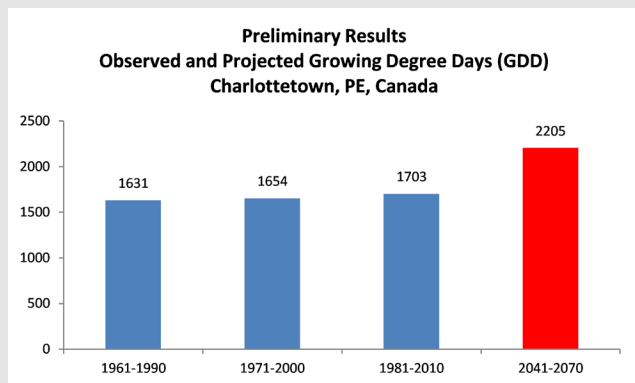
Figure 3.8: Historical observations and preliminary projections for the number of growing degree days (>5°C) in Charlottetown, PE, Canada (Source: Fenech, 2016).
