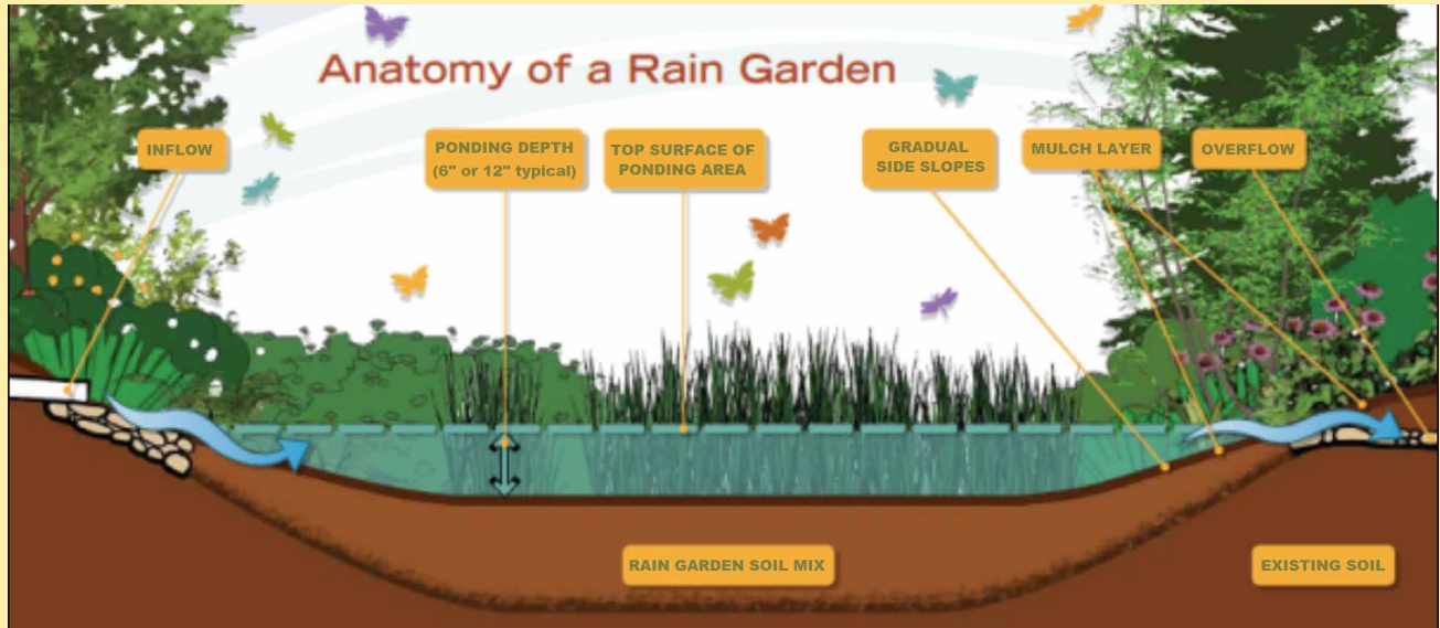
Figure 12.5: Anatomy of a rain garden (Source: http://ext100.wsu.edu/raingarden/wp-content/uploads/sites/74/2016/01/rg-schematic.png ).
